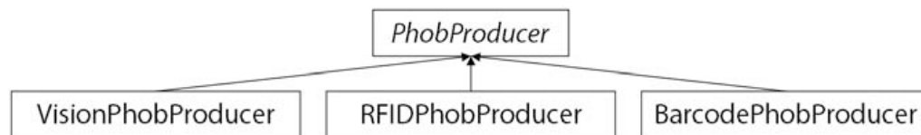
Figure 5. The inheritance hierarchy for PhobProducers. Producers are paired with InputDevices; they take input from a device and generate PhobEvents. The abstract PhobProducer base class manages the event listeners and the production of events.
